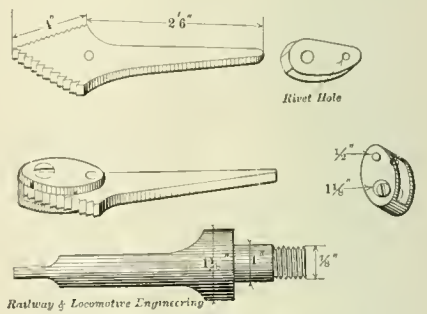
STUD WRENCH, DRILL AND REAMER.
